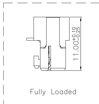
SECTION E-E
