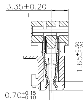
SECTION F-F
