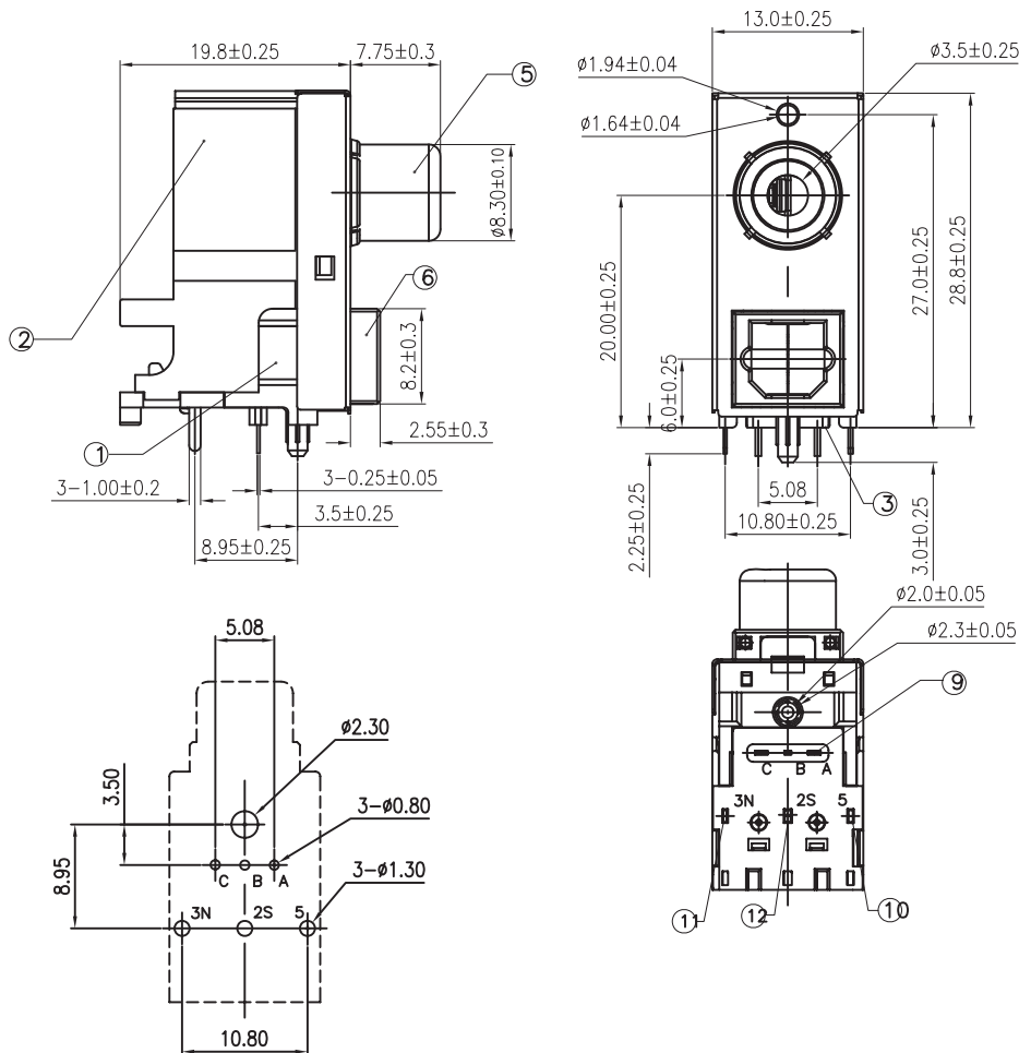
Recommended PCB Layout <BOTTOM VIEW>
