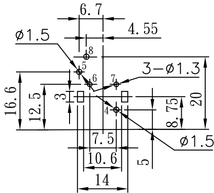
T:1.6 Dimensions of PC board holes
