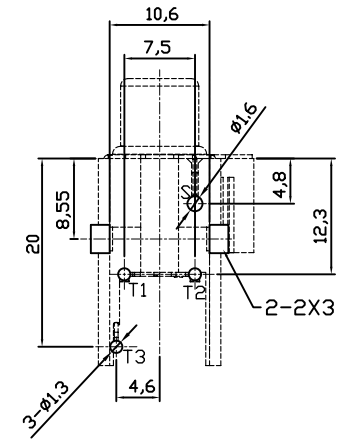
RECOMMENDED P.C.B. LAYOUT (T=1.60) TOLERANCE: ±0.05 (BOTTOM VIEW)
