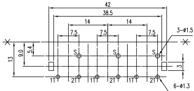
T:1.6 Dimensions of PC board holes Tolerance : ±0.1(Printed-side view)
