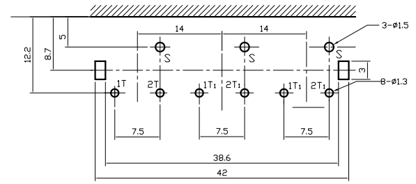
T:1.6 Dimensions of PC board holes Tolerance : ±0.1(Printed-bottom view)
