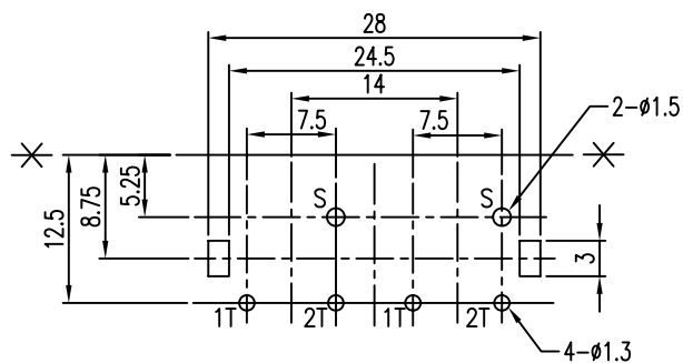
T:1.6 Dimensions of PC board holes Tolerance : \pm 0.1 (Printed-bottom view)
