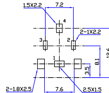
HOLE LAYOUT
