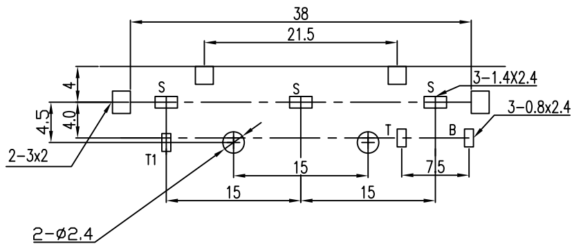
T:1.6 Dimensions of PC board holes Tolerance : ±0.1(Printed-bottom view)
