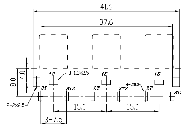
P.B.C LAYOUT BOTTOM VIEW
