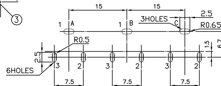
T:1.6 Dimensions of PC board holes
