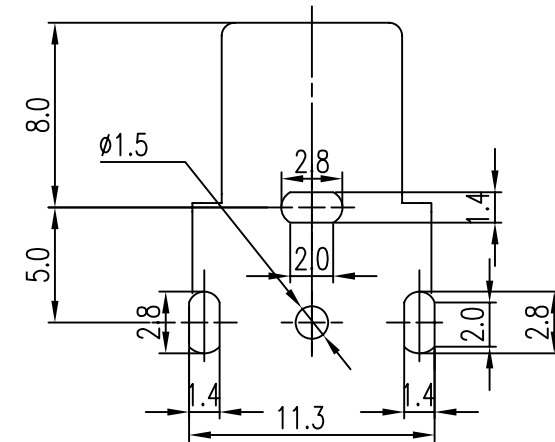
T:1.6 Dimensions of PC board holes Tolerance : \pm 0.05 (Printed-bottom view)
