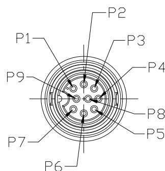
Pin Assignment
