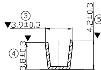
SEC. B-B
