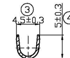
SEC. B-B
