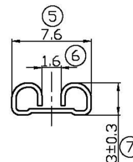
SEC. B-B
