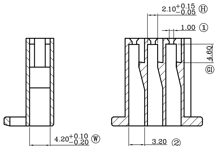
SEC B-B
