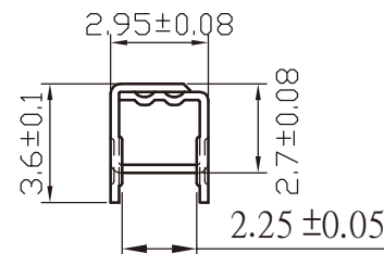
SEC.C-C
