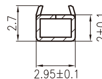
SEC.C-C
