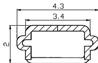
SECTION C-C 10/1
