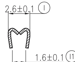
SEC C-C
