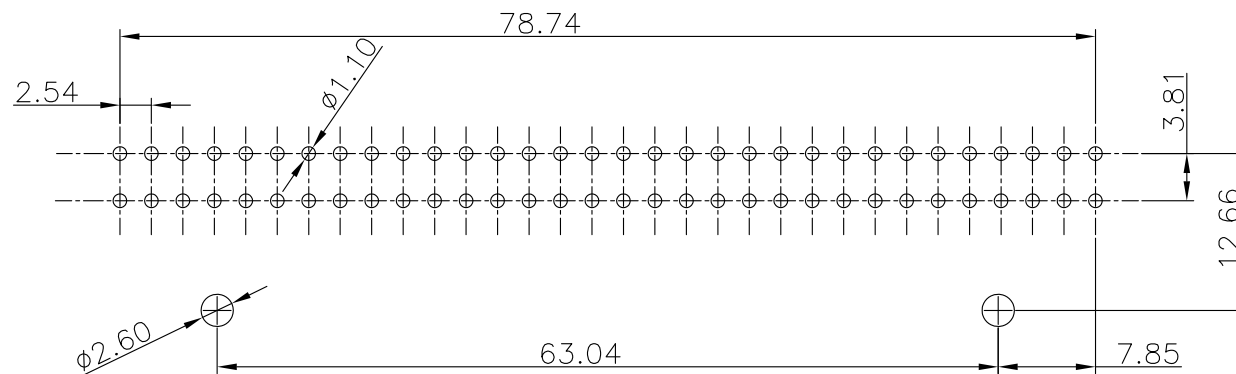
P.C. Board Layout (Tolerance:±0.05) (Top View)
