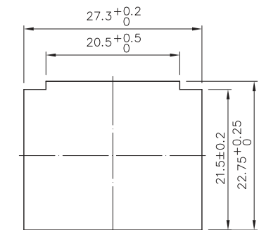
SUITABLE PANEL CUTOUT FOR 1.0 TO 2.5 PANEL THICKNESS MOUNTING HOLE
