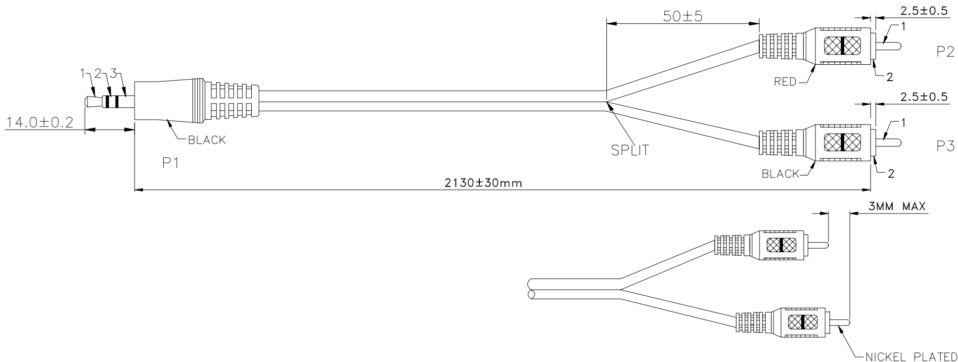
PIN OUT
