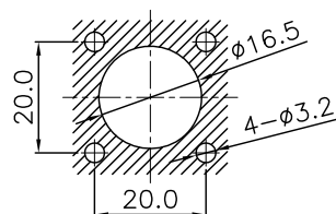
RECOMMENDED PANEL HOLE
