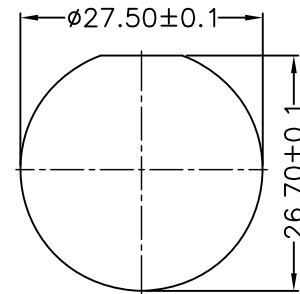
Panel Cut-Out
