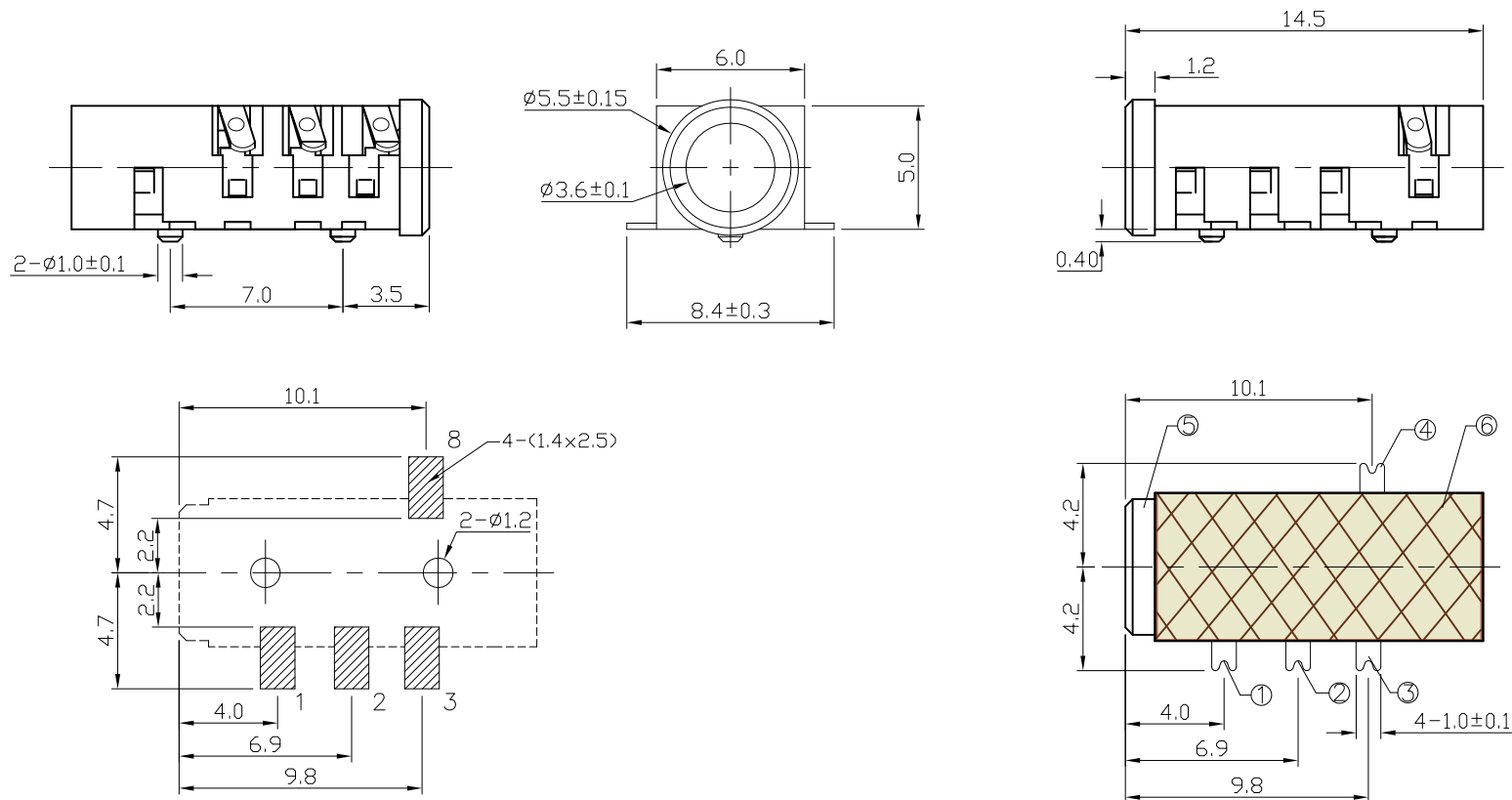
T:1.6 Dimensions of PC board holes Tolerance : \pm 0.1 (Printed-top view)
