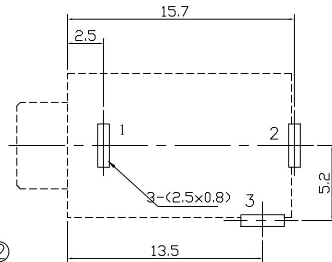
T:1.6 Dimensions of PC board holes Tolerance : \pm 0.05 (Printed-top view)
