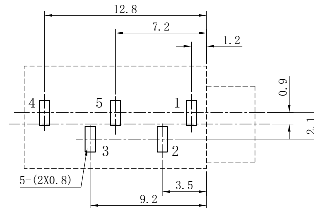
T:1.6 Dimensions of PC board holes
