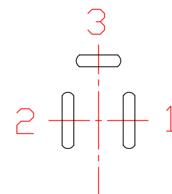
Pin Hole Layout (Jack Bottom View)
