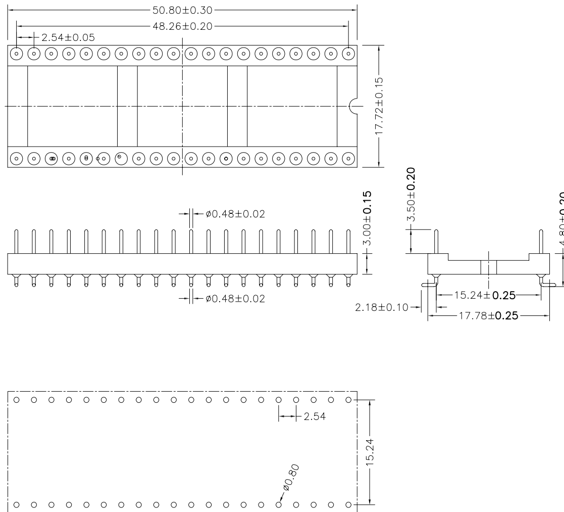
P. C. B LAYOUT
