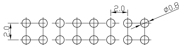
RECOMMENDED P.C. BOARD HOLE DIMM.
