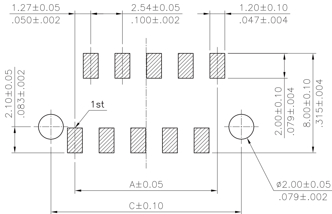
P.C.B Layout Clearance Fit With P.C.B Pegs
