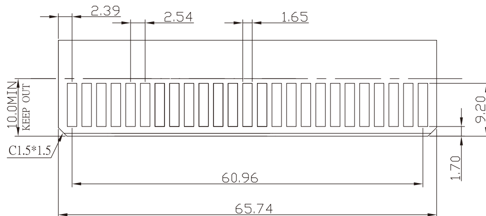
RECOMMENDED MATTING BOARD FOOTPRINT (Tolerance: \pm 0.05 )
