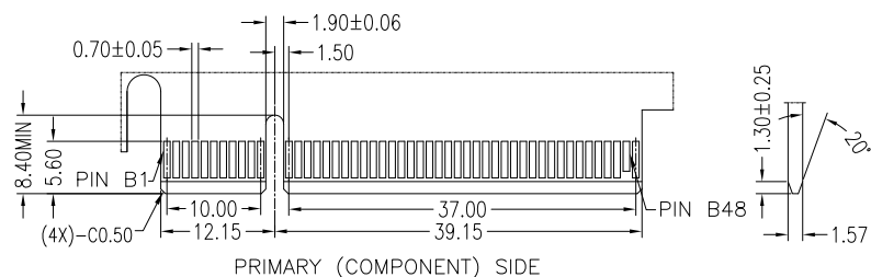
PRIMARY (COMPONENT) SIDE
