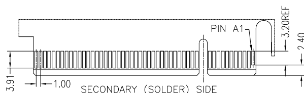
SECONDARY (SOLDER) SIDE
