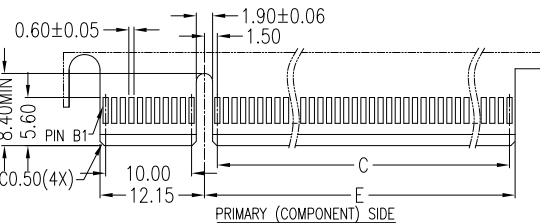
ADD-IN CARD EDGE-FINGER DIMENSIONS DEFAULT TOLERANCE ±0.13
