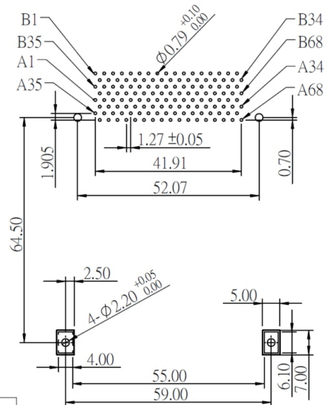
PCB LAYOUT
