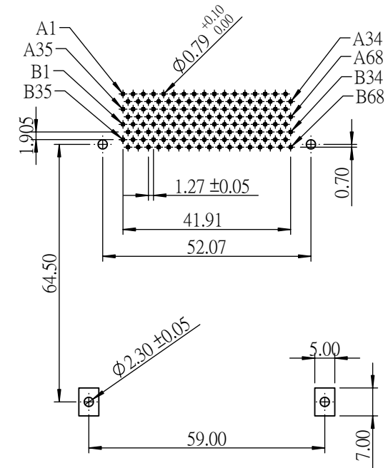
PCB LAYOUT : COMPONENT SIDE
