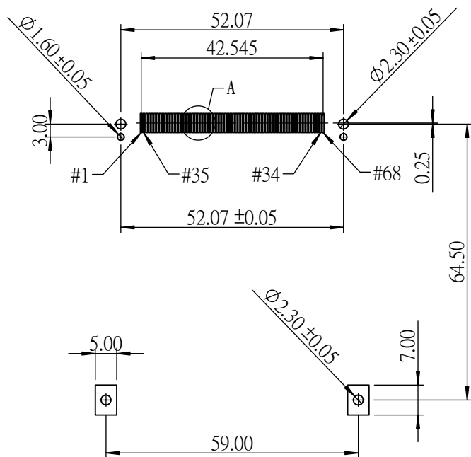
PCB LAYOUT : COMPONENT SIDE
