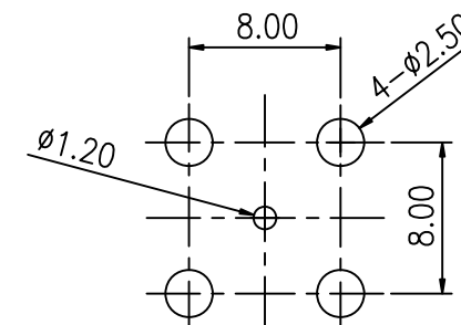
RECOMMENDED MOUNTING PCB HOLE
