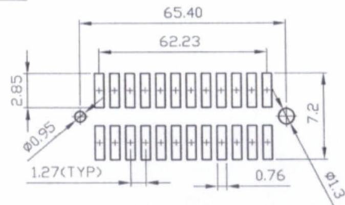
Recommended P.C. Board hole layout
