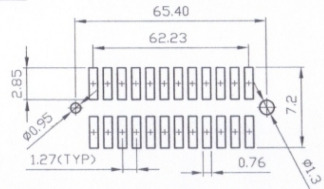
Recommended P.C. Board hole layout
