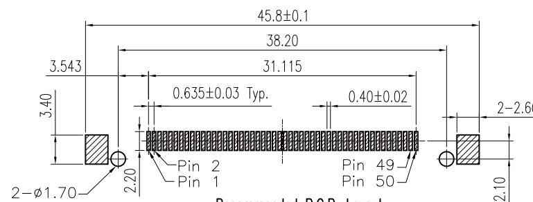
Recommended P.C.B. Layout Layout Tolerance = ± 0.05 mm
