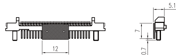
With Cap Scale 1:1
