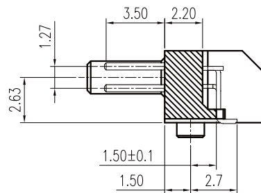
Section B-B Scale 3.2:1
