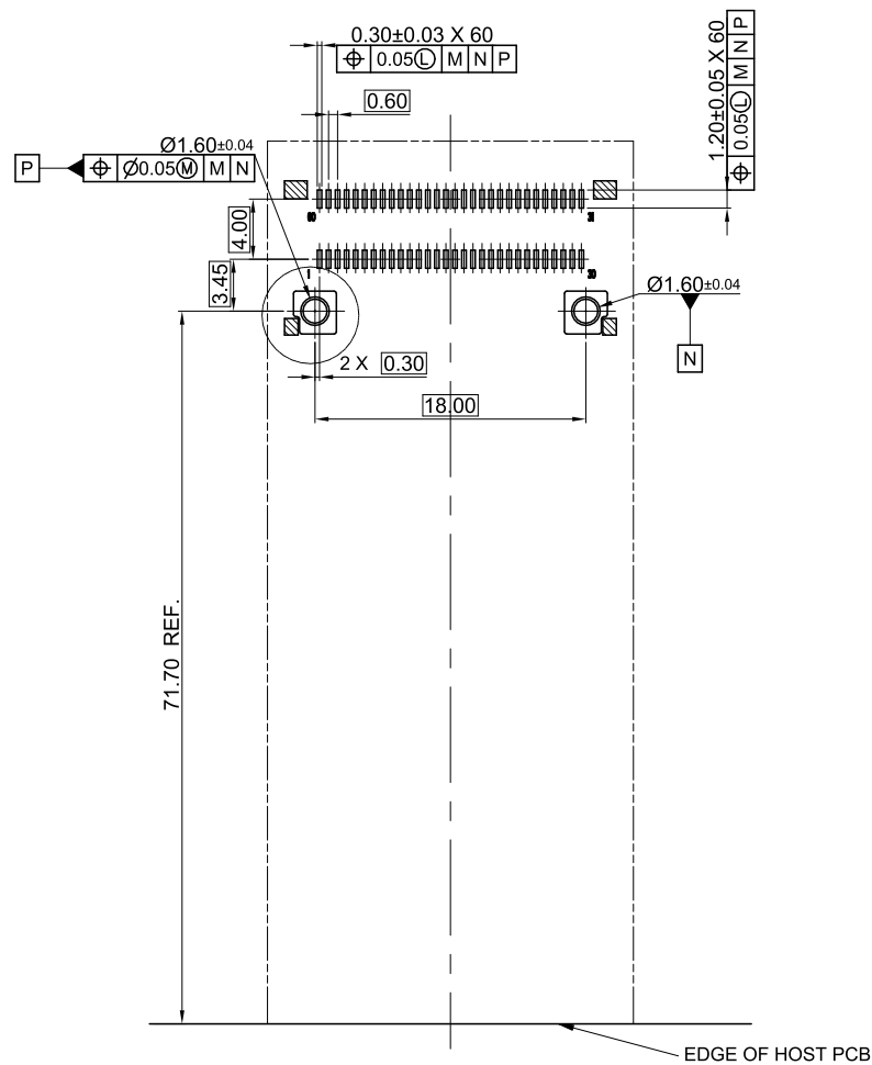
MOTHERBOARD FOOTPRINT RECOMMENDATION
