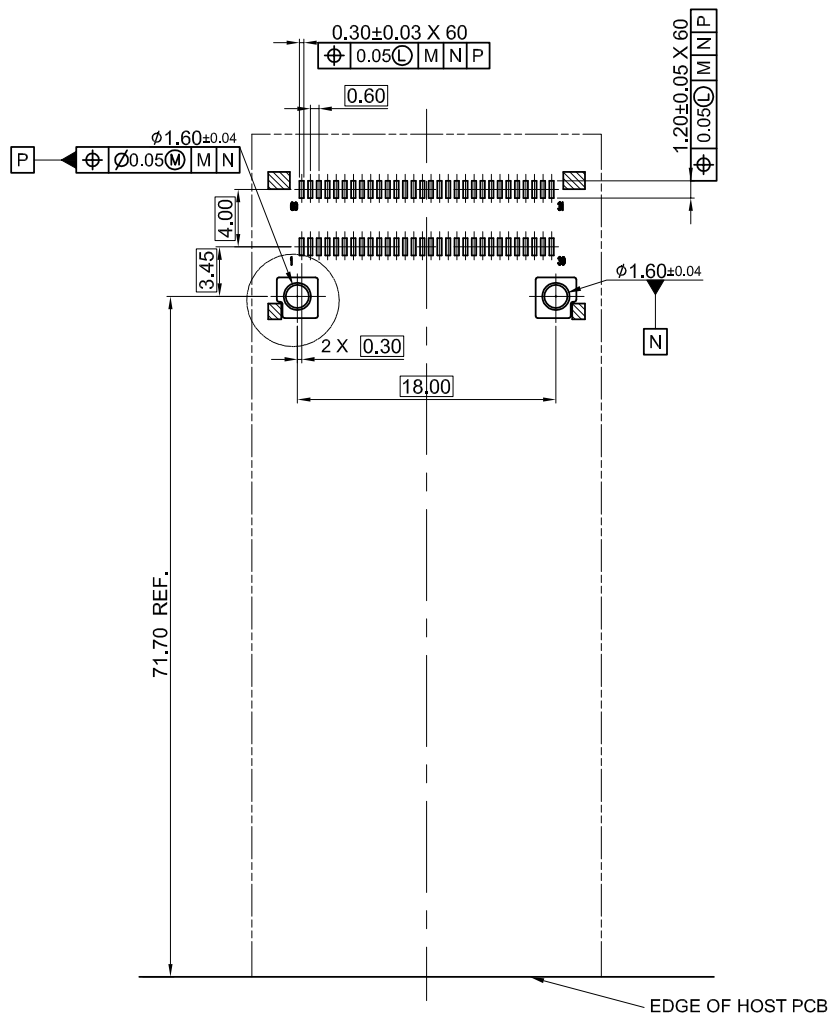
MOTHERBOARD FOOTPRINT RECOMMENDATION
