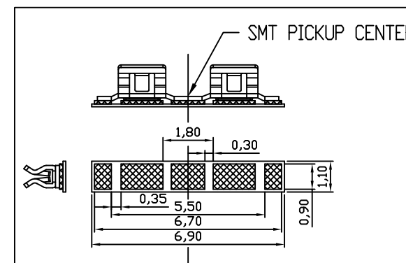
PCB Recommend Layout Pattern
