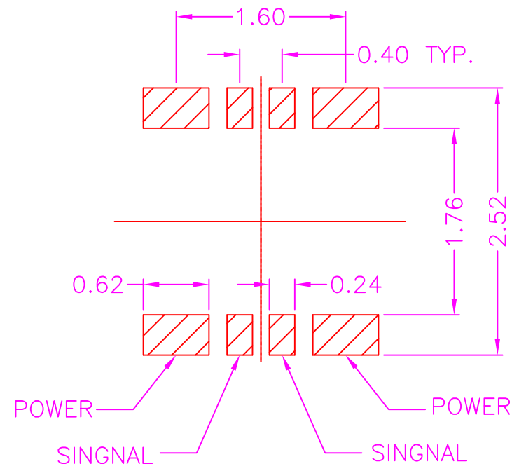
P.C.B. LAYOUT TOP VIEW \pm 0.05
