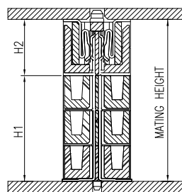
MATING HEIGHT
