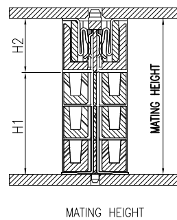
MATING HEIGHT
