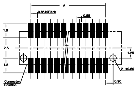
PCB Layout For Surface Mount
