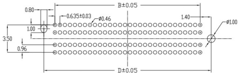
Recommended PC board pattern (TOP VIEW)
